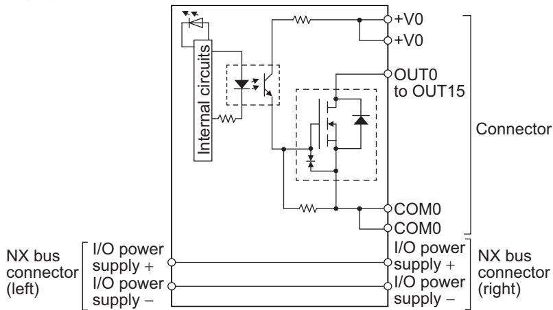
CN1 (left) output circuit
