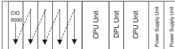
Duplex CPU System, CPU Rack
