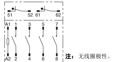
G7Z-3A1B-02Z
