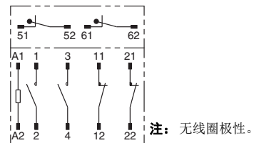
G7Z-2A2B-02Z
