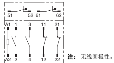
G7Z-2A2B-02Z-R
