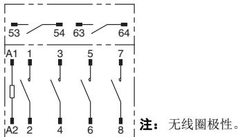
G7Z-3A1B-20Z
