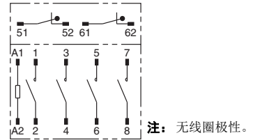
G7Z-3A1B-02Z-R
