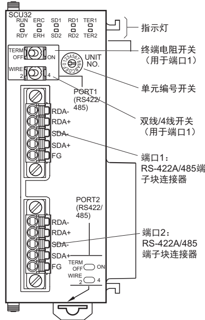
CJ1W-SCU32
